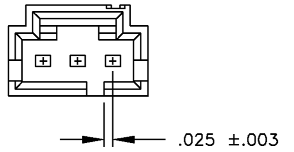
DETAIL FOR -2 ONLY (3 POSITION)
